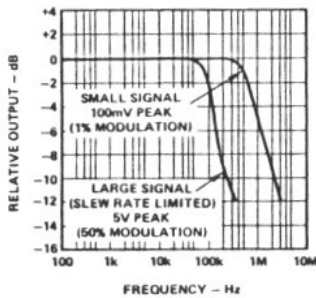
Reference Amplifier Input Frequency Response
