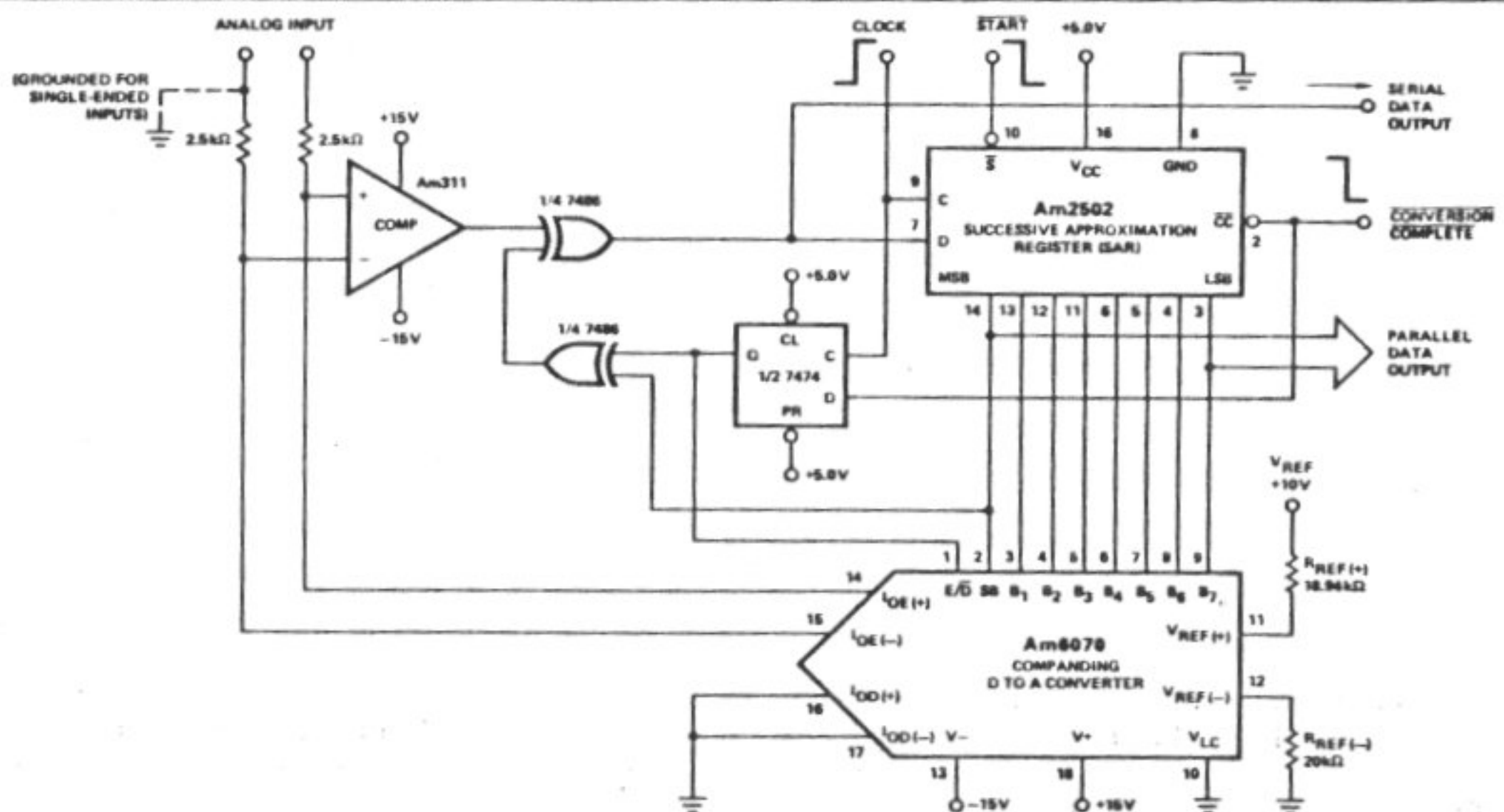
Figure 3. Detailed Encoder Connections.
