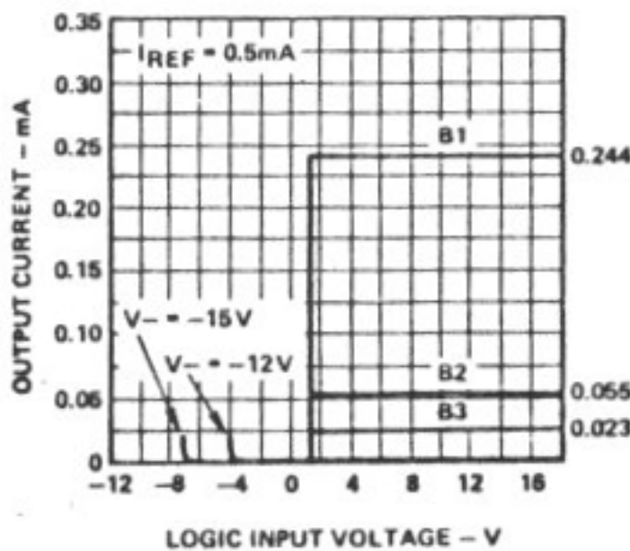
Bit Transfer Characteristics (Note 10)
