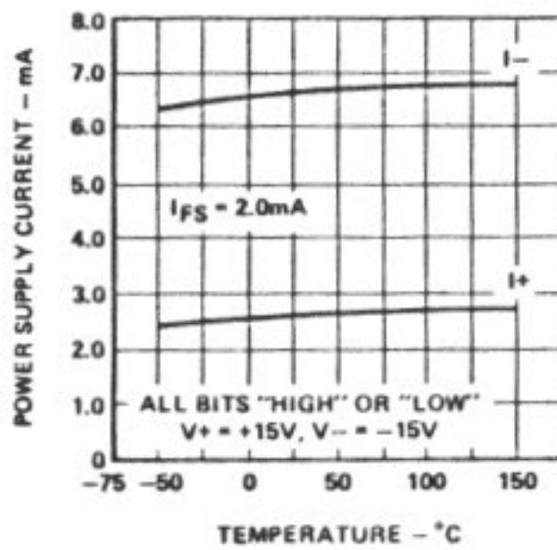
Power Supply Currents Versus Temperature
