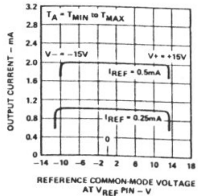
Reference Amplifier Input Common-Mode Range (Note 9)
