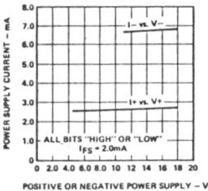
Power Supply Currents Versus Power Supply Voltages
